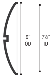
Side frame
